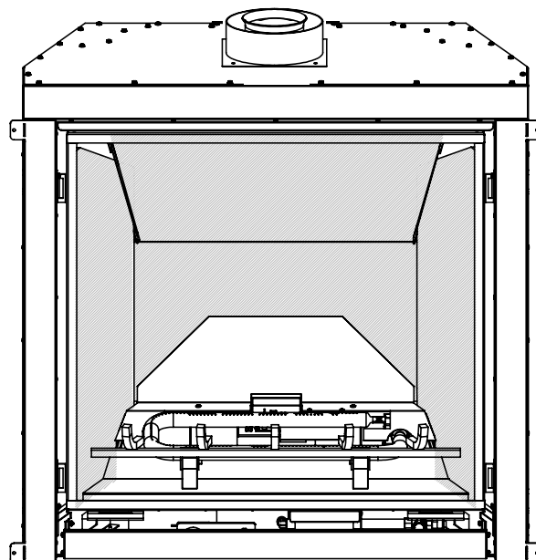
Figure 3. Liner panel position
