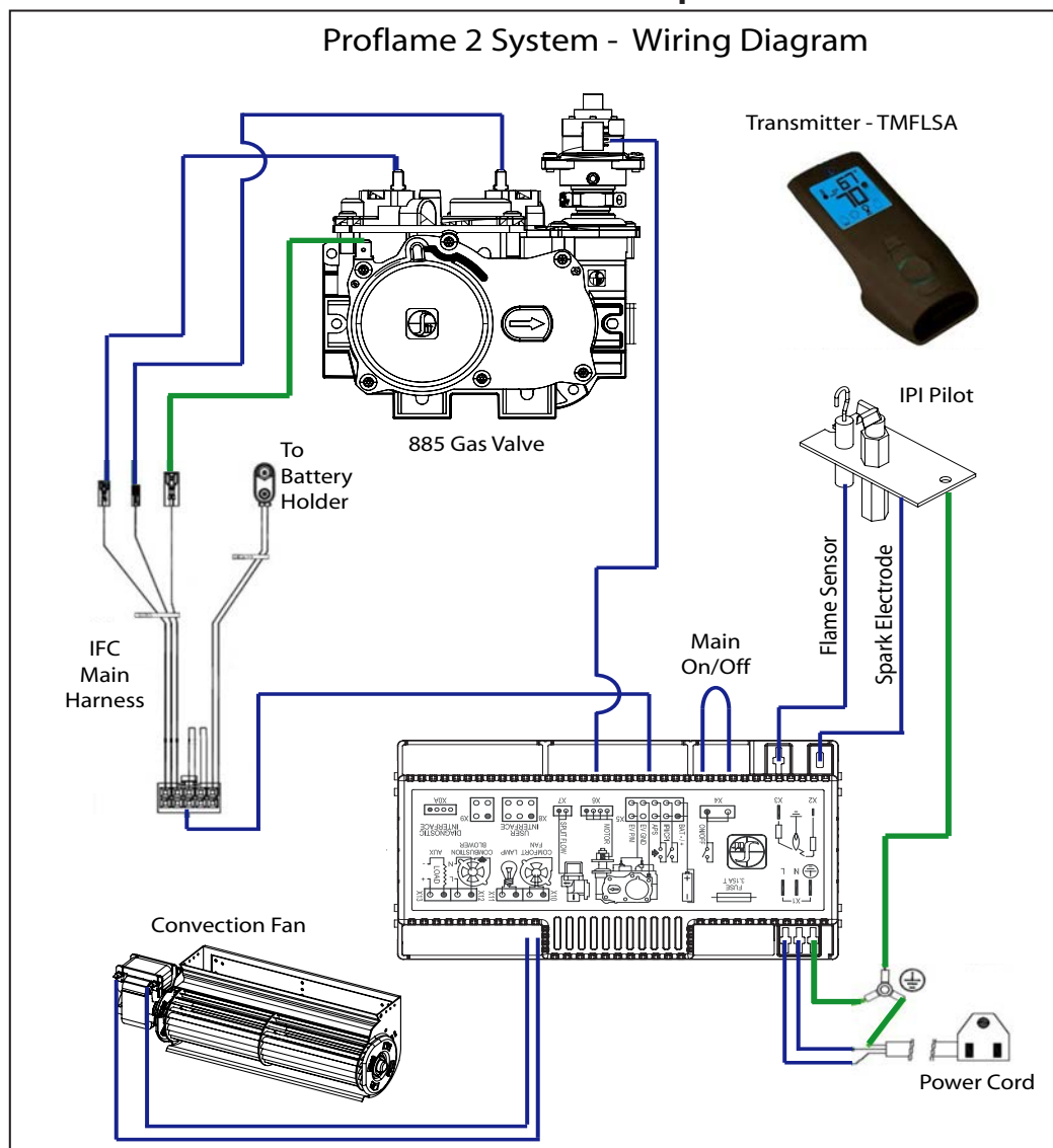
Figure 44: Wiring Diagram
