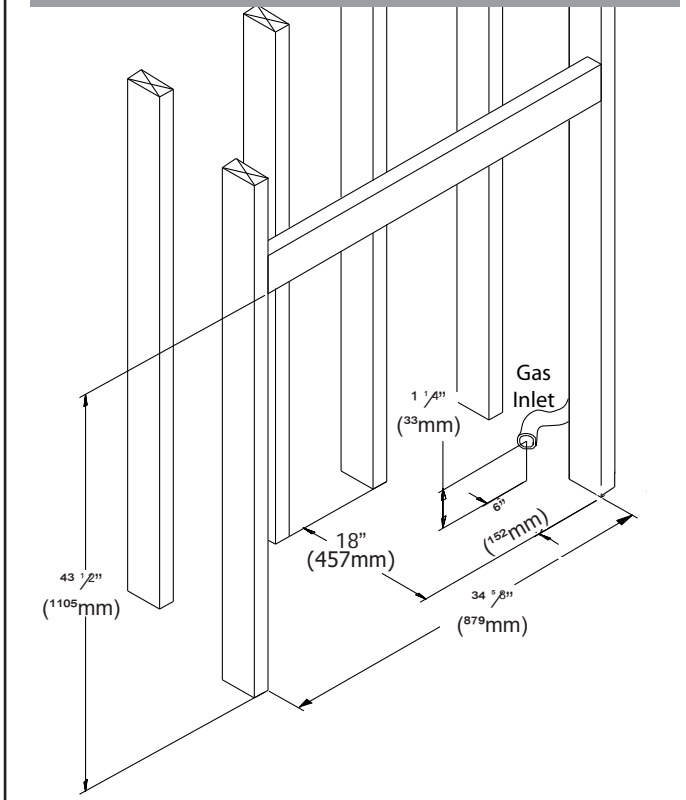
Figure 28: Construction Framing Dimensions
