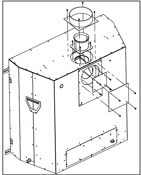
Figure 25. Top to Rear Vent Conversion
